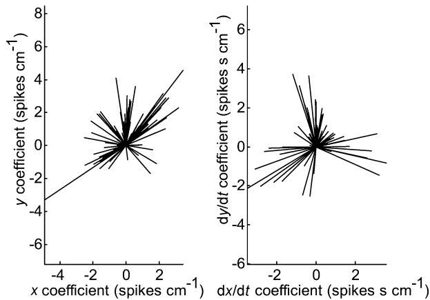
Figure 5. Preferred directions in position and velocity space are given by the coefficients from the encoding model using coefficients in Cartesian coordinates from a random data set All illustrated units had a VAF > 40%. Note the wide range of preferred directions for both the position (left panel) and the velocity (right panel) coefficients.
