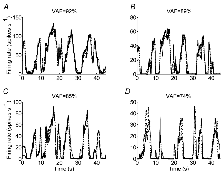
Figure 6. Comparison of the actual (line) and predicted firing rates (dots) for the best fitting (A) the 3rd best (B), the 10th best (C) and the 30th best fitting neurone (D) The VAF (%) is shown for each unit.
