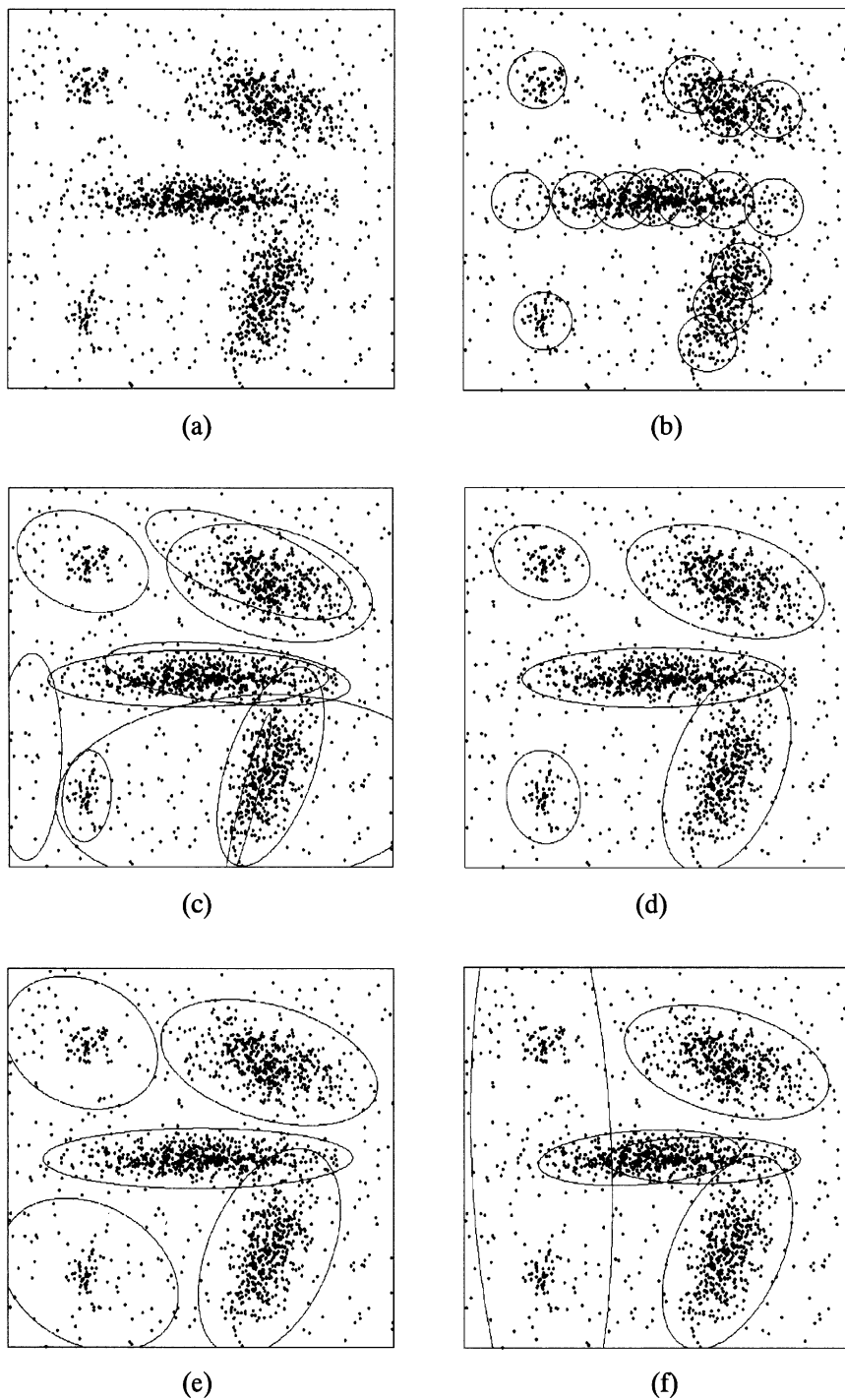
Fig. 2. Results with ellipsoidal clusters and uniform noise (a) Raw data. (b) Initialization. (c) Results at \beta = 0.83 ( v^* = 2.7 ). (d) Convergence at \beta = 0.64 ( v^* = 1.6 ). (e) Final result, \beta = 1 ( v^* = 3.9 ). (f) Spurious solution obtained by EM.
